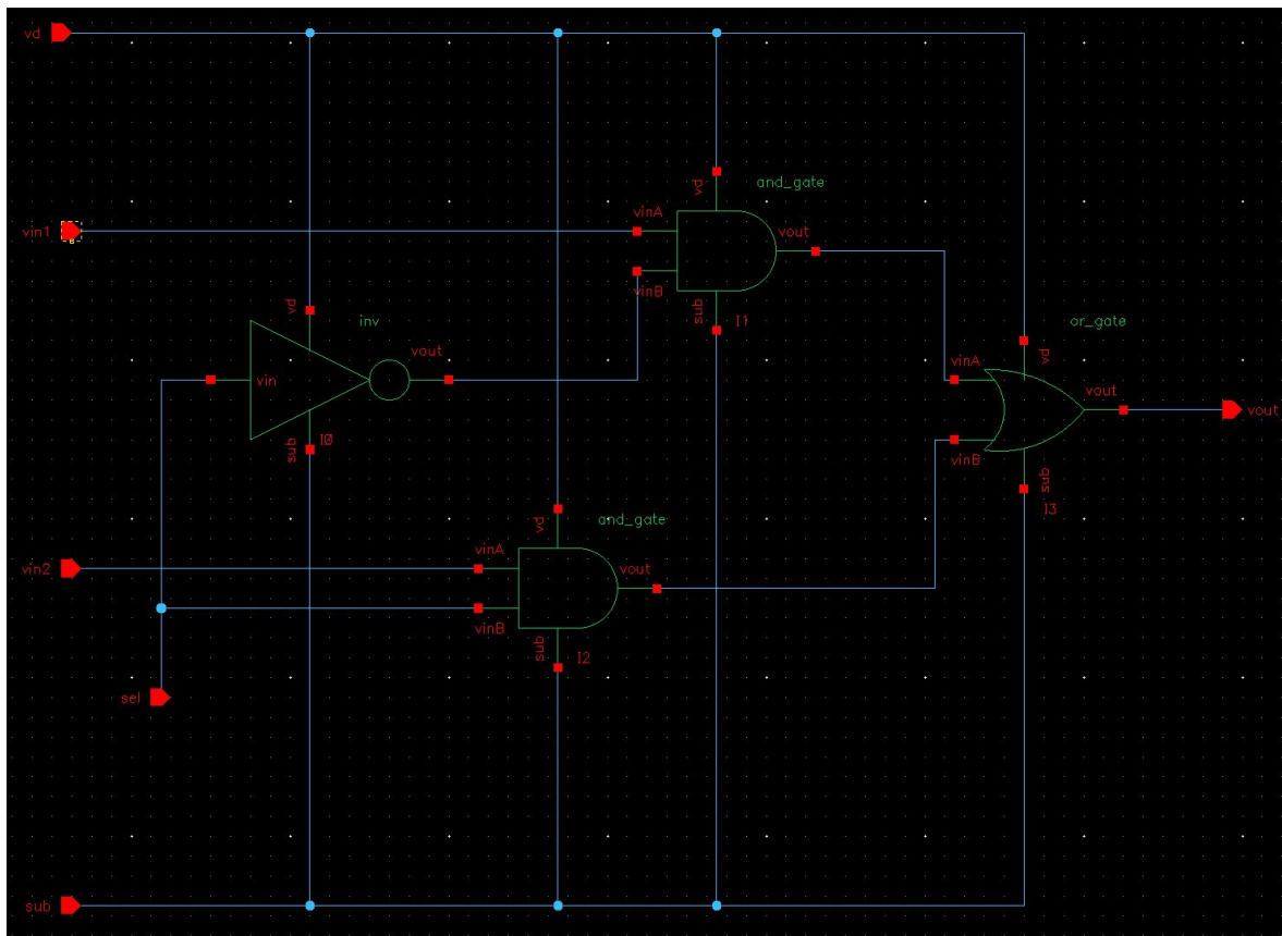
2-to-1 mux Schematic
